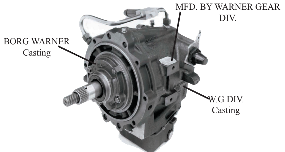
Borg Warner / Velvet Drive 1016 Transmission
